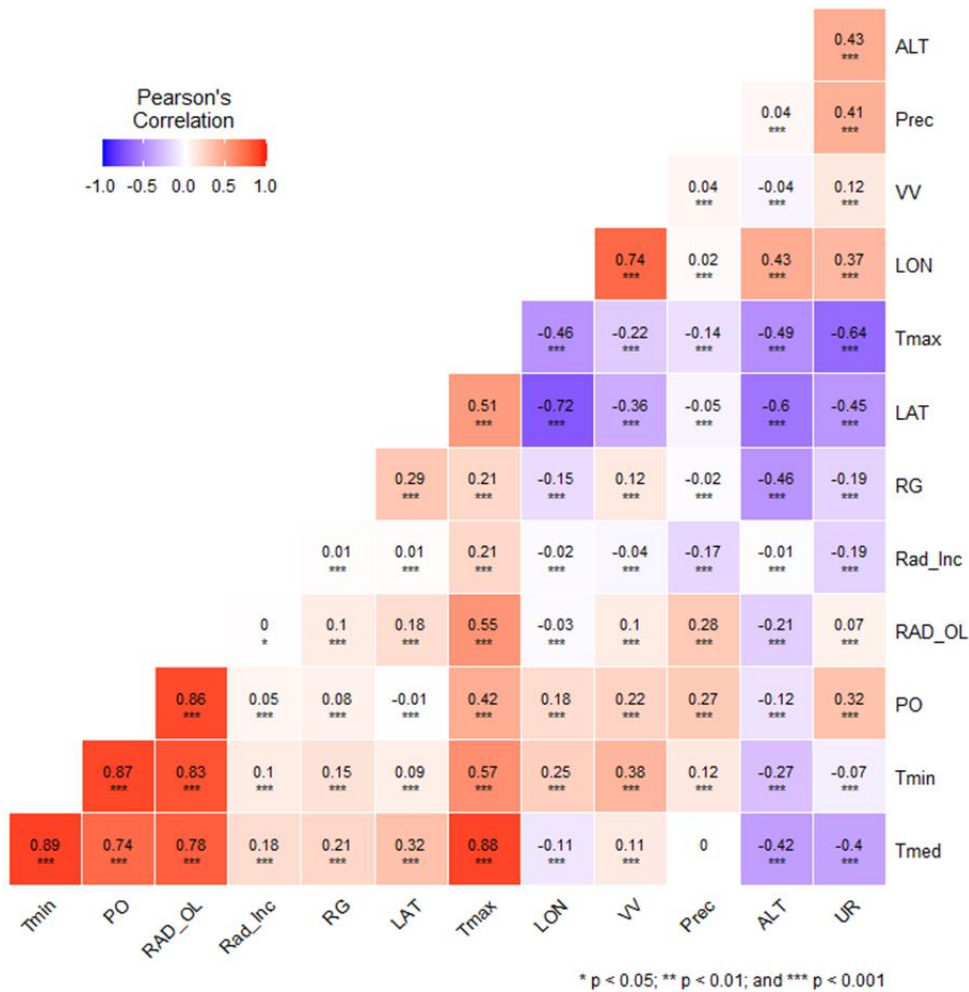
Figure 2. Pearson's linear correlation between soybean grain yield (GY) and altitude (ALT), longitude (LON), latitude (LAT), precipitation (Prec), wind speed (W), incident radiation (Rad_Inc), total radiation RAD_OL, dew point (PO), minimum temperature (Tmin), average temperature (Tavg), maximum temperature (Tmax), and relative air humidity (RH).
